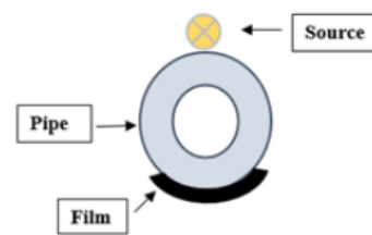
Fig.4. The DWSI technique
