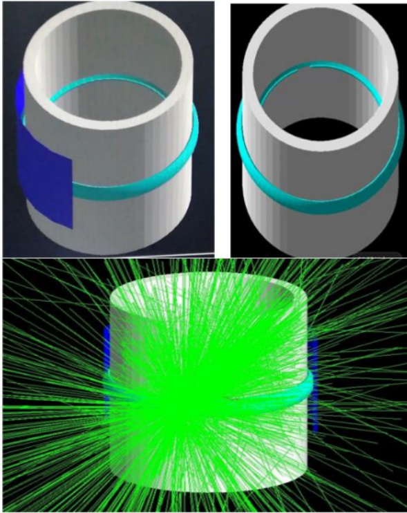
Fig. 5. The carbon steel pipe setup in GATE. The cyan region represents the weld, and the blue curved volume represents the film.
