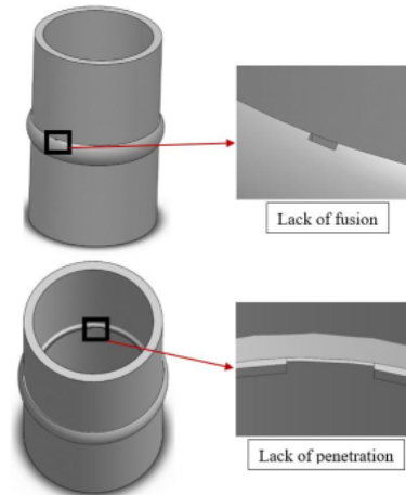
Fig.2. The 4-inch diameter Carbon steel pipe.
