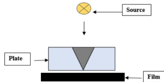
Fig.3. The SWSI technique
